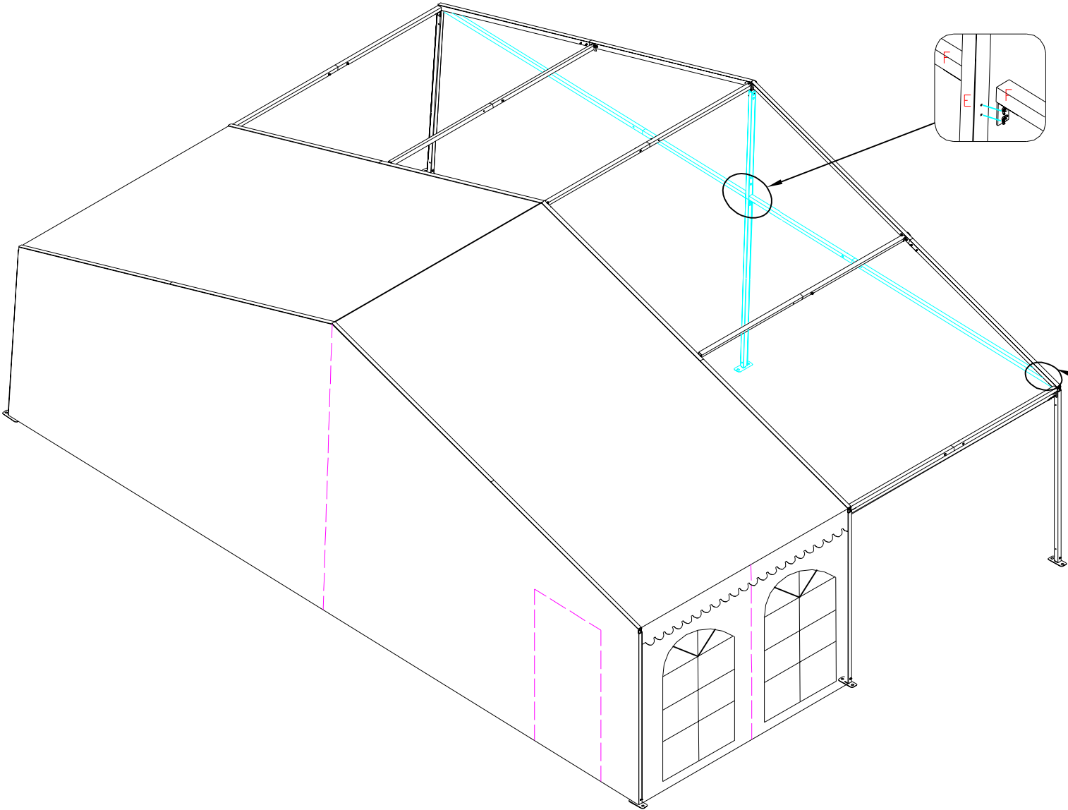
Step 16 Side eaves and gable pole connections
