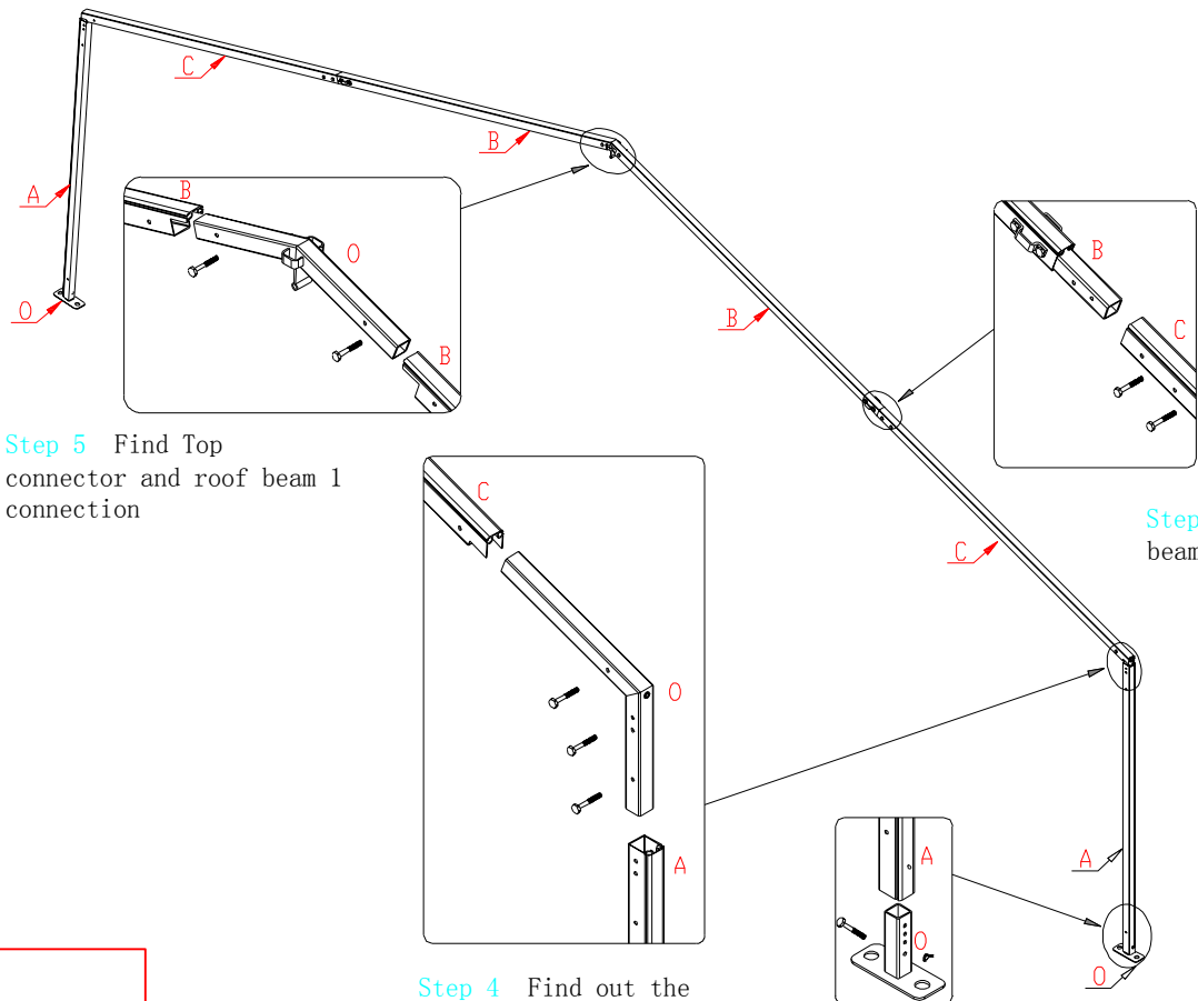
Step 4 Find out the Corner connector and leg, Roof beam 2 connections
