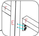
Step 16 Side eaves and gable pole connections
