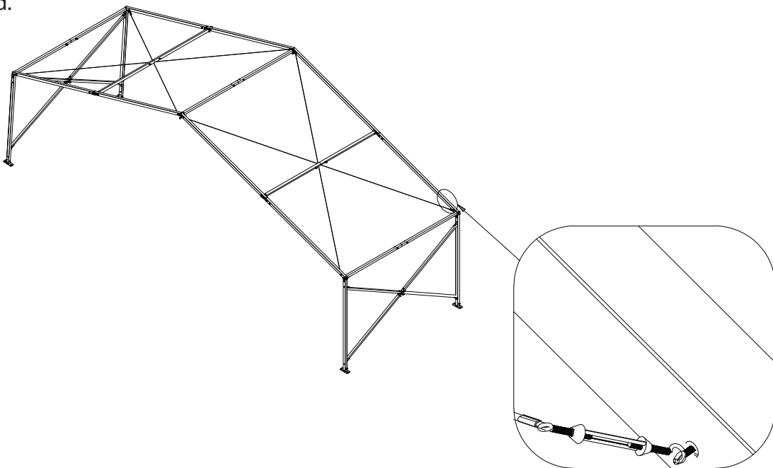
Step 11 Installation of Roof Cover Wire, elastic adjustment screws
